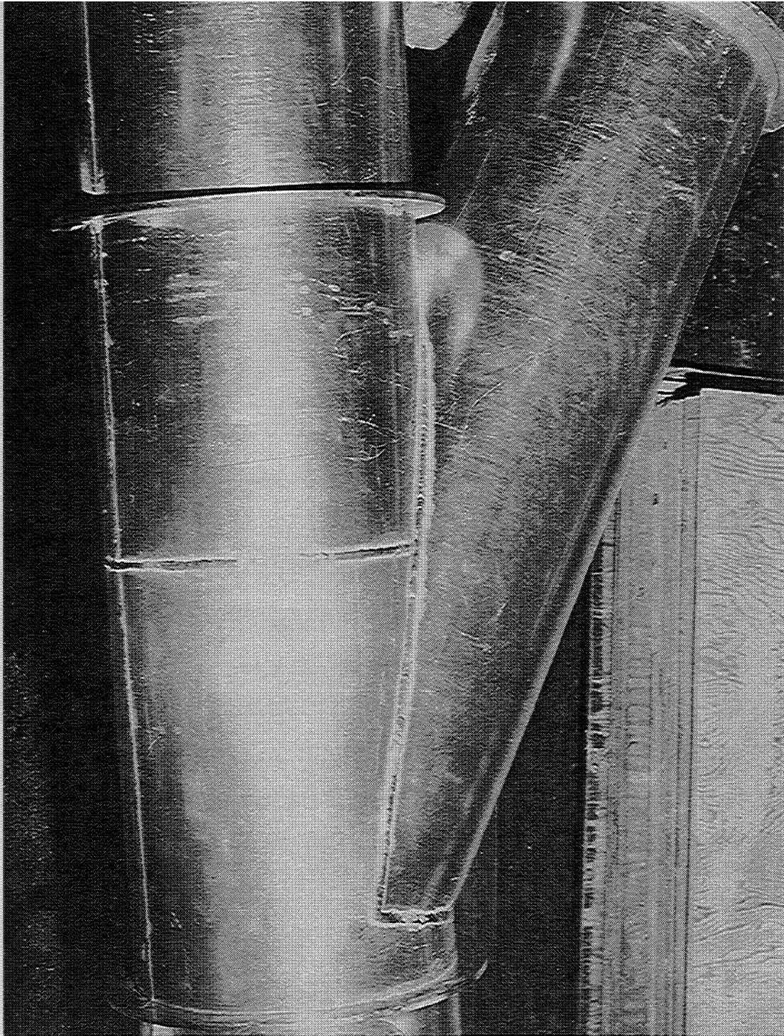
Fig. 1. The Region of Intersection of the Two Aluminum Cylinders Forming the 30^\circ Lateral.
