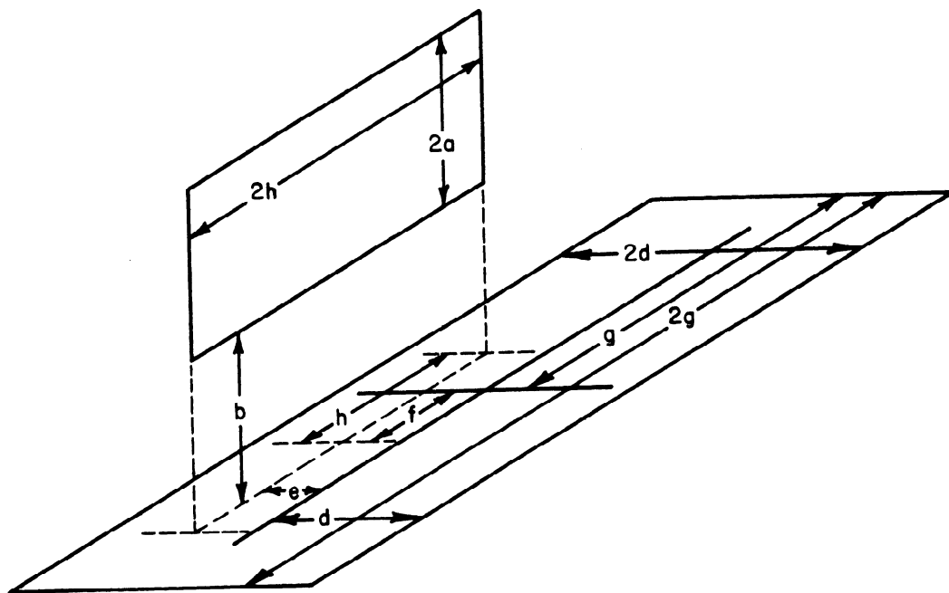
FIG. 5.3 INTERACTION BETWEEN PERPENDICULAR RECTANGLES (The 2g and 2h edges are parallel)
