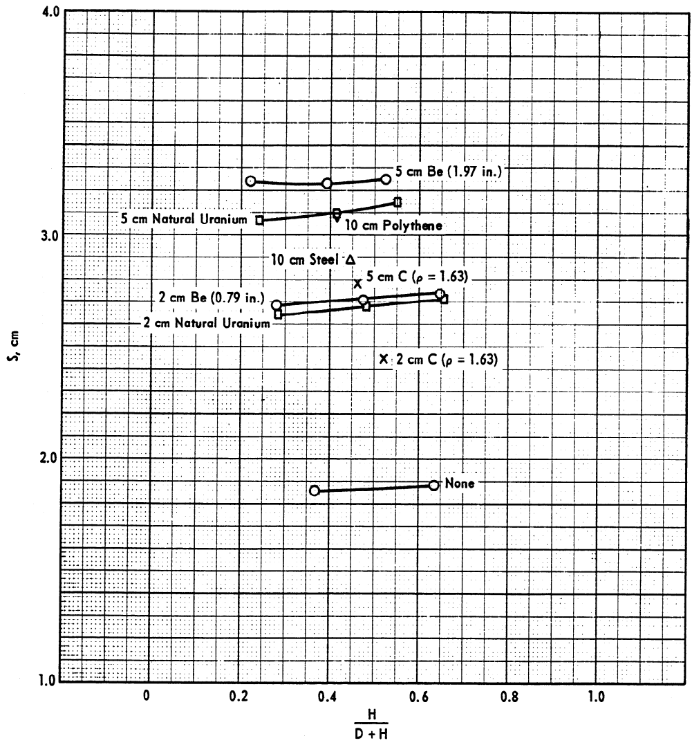
FIG. 2.12 REFLECTOR SAVINGS OF MATERIALS FOR CYLINDERS OF \delta -PHASE PLUTONIUM
