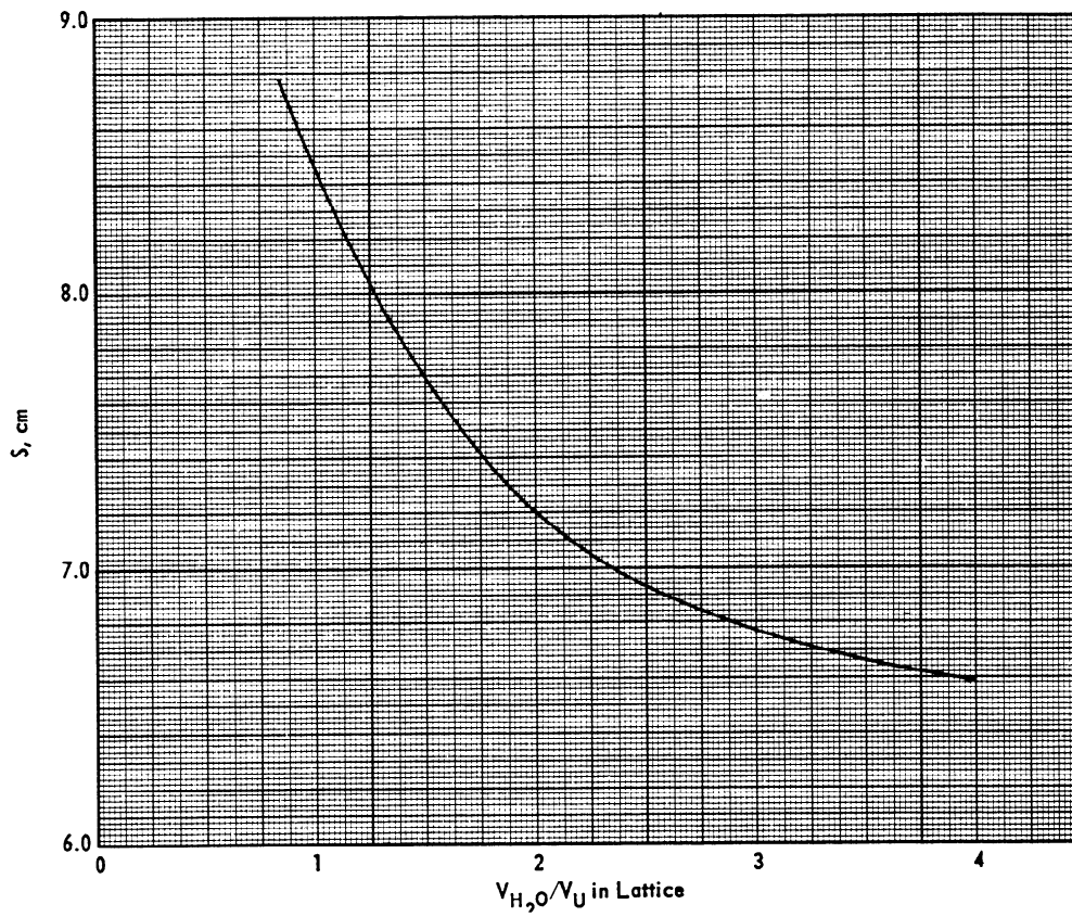
FIG. 3.4 REFLECTOR SAVINGS FOR LATTICES OF URANIUM ( < 5\% \text{ U}^{235} ) RODS IN WATER (The arrays are cylindrical and the thickness of the water reflector is effectively infinite.)
