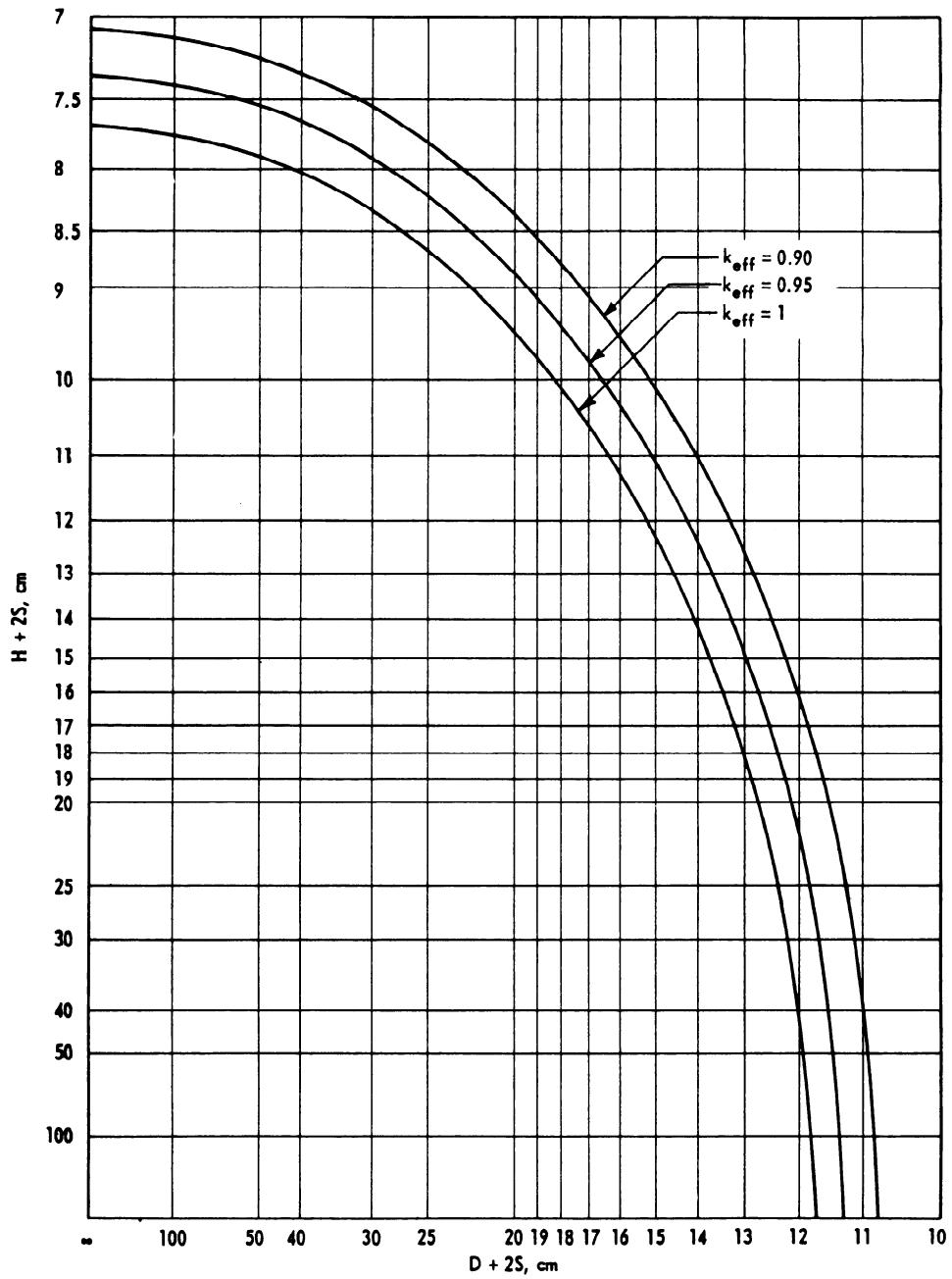
FIG. 2.15 DIMENSIONS OF A U^{233} CYLINDER AS A FUNCTION OF S AND k_{eff}
