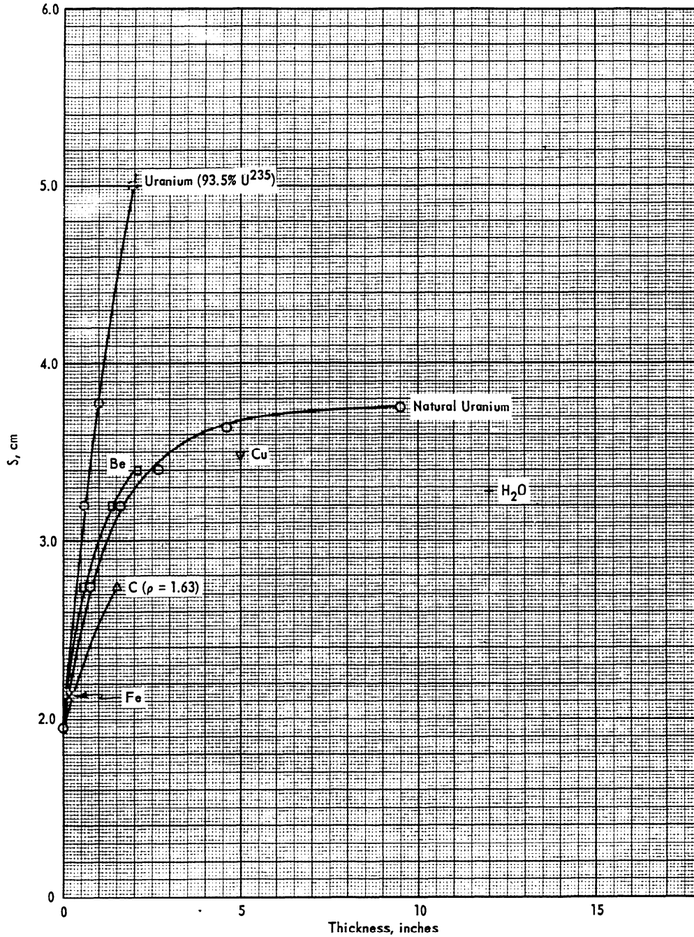
FIG. 2.10 REFLECTOR SAVINGS OF MATERIALS FOR \delta -PHASE (\rho = 15.8 \text{ g/cm}^3) PLUTONIUM
