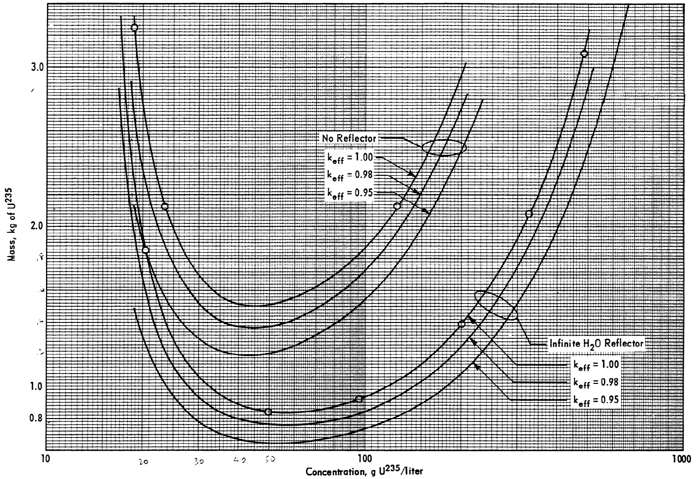
FIG. 4.4 DEPENDENCE OF MASSES OF U^{235} IN SPHERES OF UO_2F_2 SOLUTION ON CONCENTRATION AND k_{eff}
