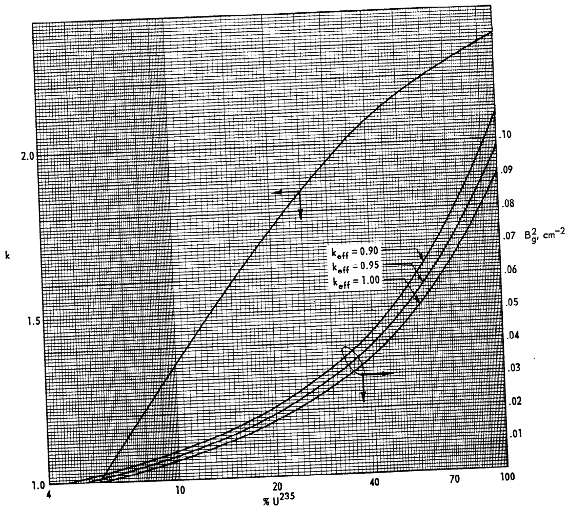
FIG. 2.6 MULTIPLICATION CONSTANT AND BUCKLING OF URANIUM AS A FUNCTION OF THE U^{235} CONCENTRATION
