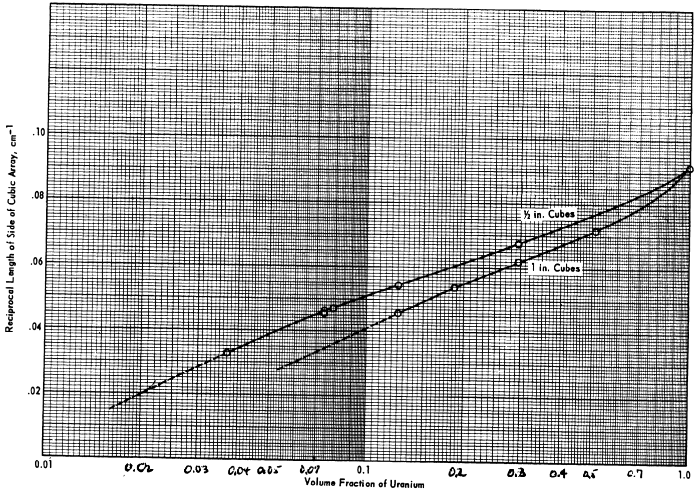
FIG. 3.1 CRITICAL SIZE OF CUBIC ARRAYS OF CUBES OF URANIUM (~94.4% U 235 ) IN WATER
