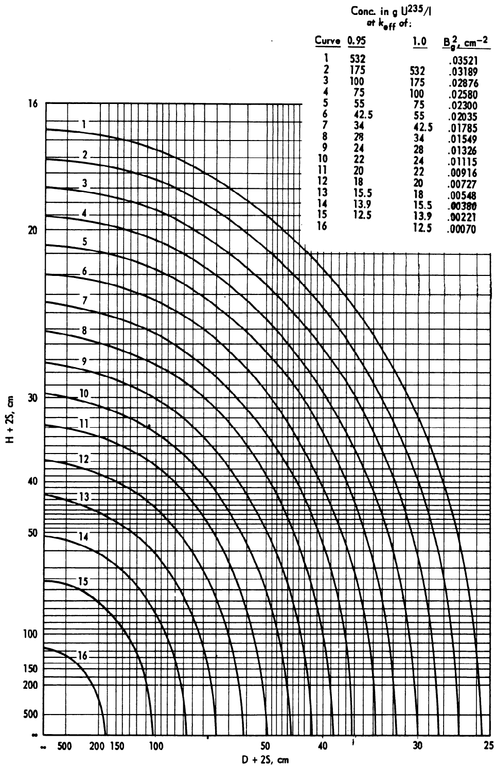
FIG. 4.7 DEPENDENCE OF SAFE ( k_{\text{eff}} = 0.95 ) AND CRITICAL ( k_{\text{eff}} = 1.0 ) DIMENSIONS OF CYLINDERS OF \text{UO}_2\text{F}_2 SOLUTION ON S AND CONCENTRATION
