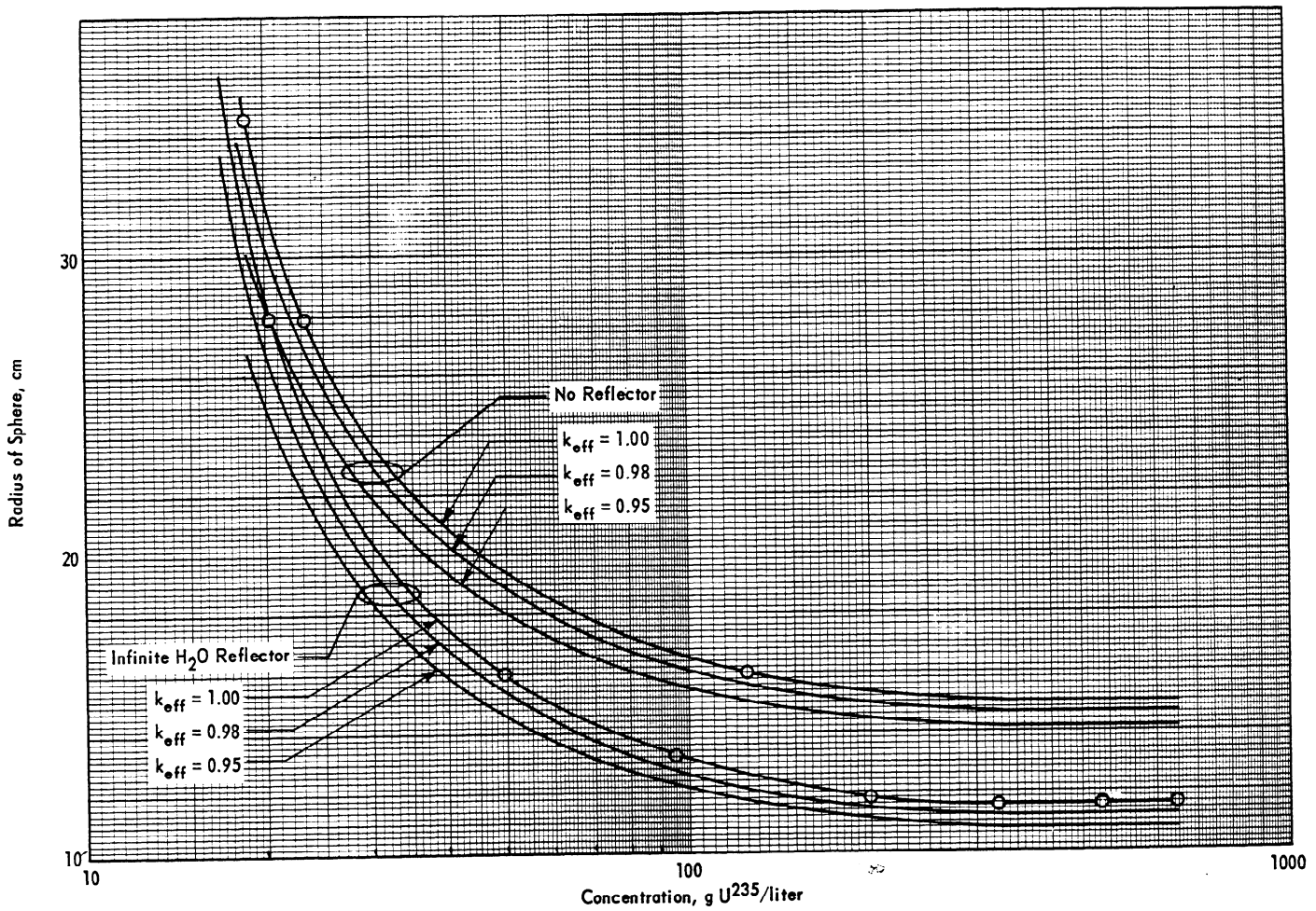
FIG. 4.5 DEPENDENCE OF RADII OF SPHERES OF \text{UO}_2\text{F}_2 SOLUTION ON CONCENTRATION AND k_{\text{eff}}
